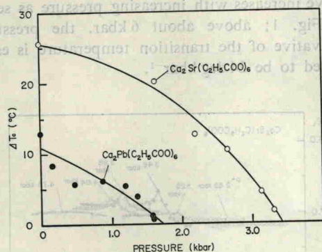
Fig. 3. Hydrostatic-pressure dependence of the thermal hysteresis \Delta T_c of the II-III transitions in \text{Ca}_2\text{Sr}(\text{C}_2\text{H}_5\text{COO})_6 and in \text{Ca}_2\text{Pb}(\text{C}_2\text{H}_5\text{COO})_6 .
