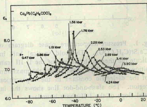
Fig. 5. Temperature dependence of the dielectric constant along the c -axis of \text{Ca}_2\text{Pb}(\text{C}_2\text{H}_5\text{COO})_6 at various hydrostatic pressures in the vicinity of the critical point. Frequency: 1 kHz.
