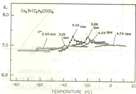
Fig. 2. Temperature dependence of the dielectric constant along the c -axis of \text{Ca}_2\text{Sr}(\text{C}_2\text{H}_5\text{COO})_6 at various hydrostatic pressures in the vicinity of the critical point. Frequency: 1 kHz.
